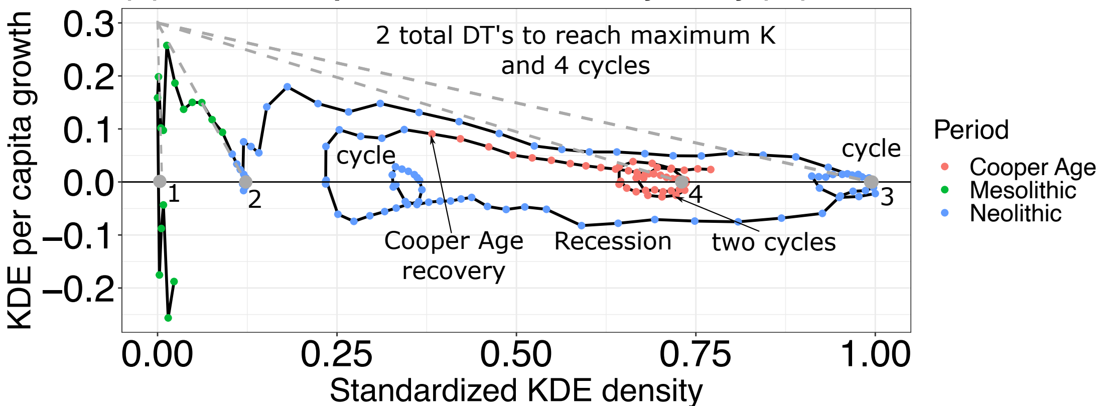
(C) KDE Per Capita Growth vs. Density – Italy (24)
